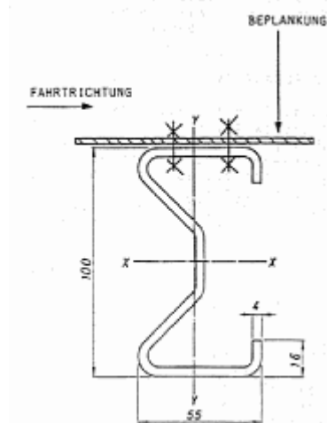
Fig. 2: Sigma guardrail post cross section
